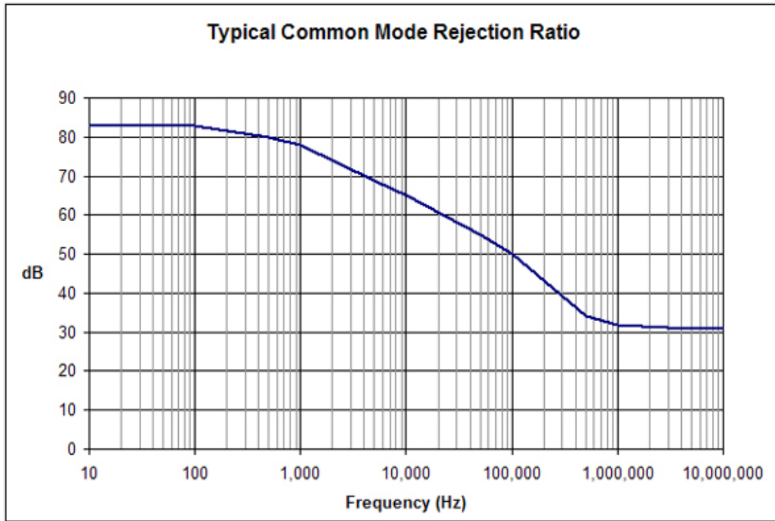
Typical CMRR vs. Frequency
