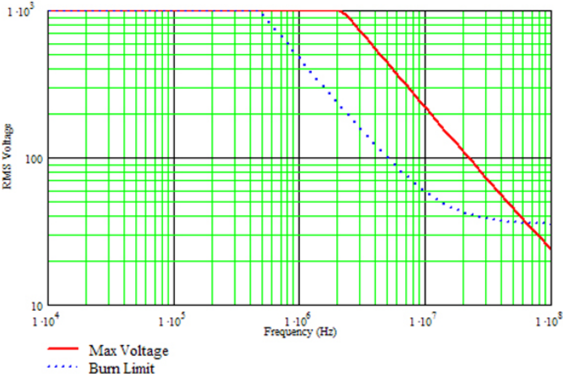
Input Voltage & Burn Limit vs. Frequency
